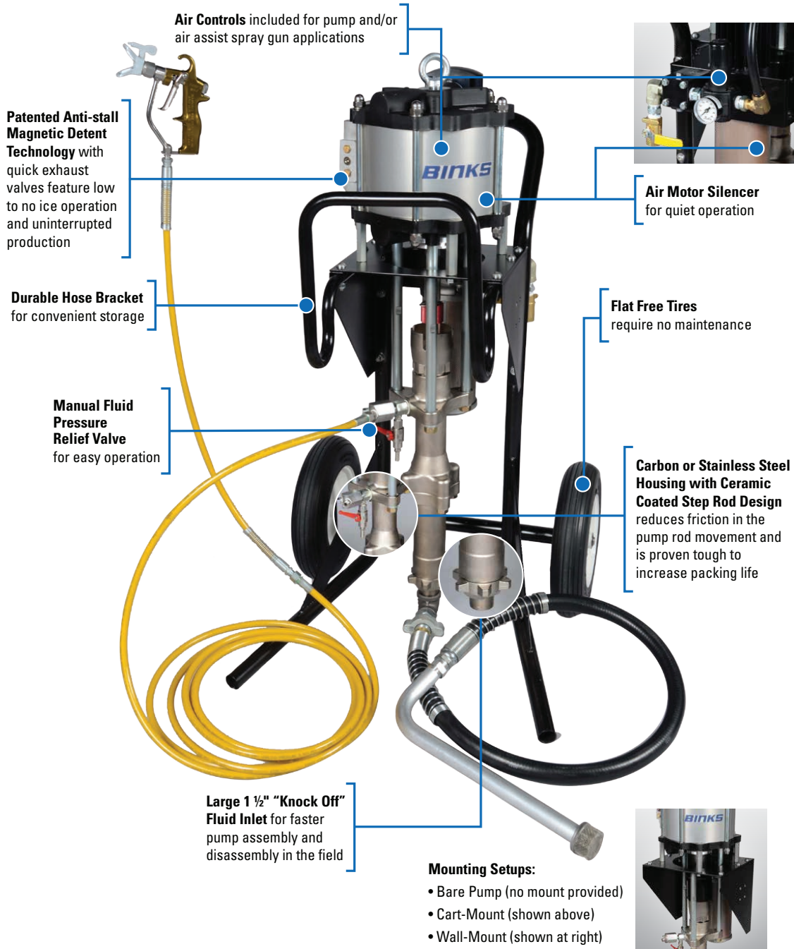
Shown: Binks MX Cart-Mount Outfit with Airless 75 spray gun, 25' airless hose, 5' whip hose and 5 gal. siphon kit.
