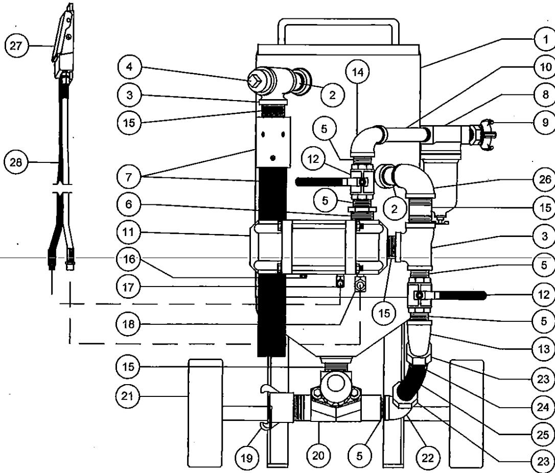
1" Piping with Combo-Micro Valve
